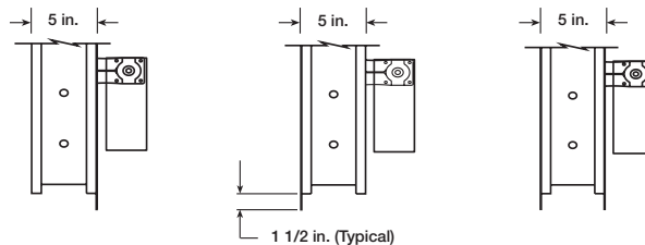
Single Flange
